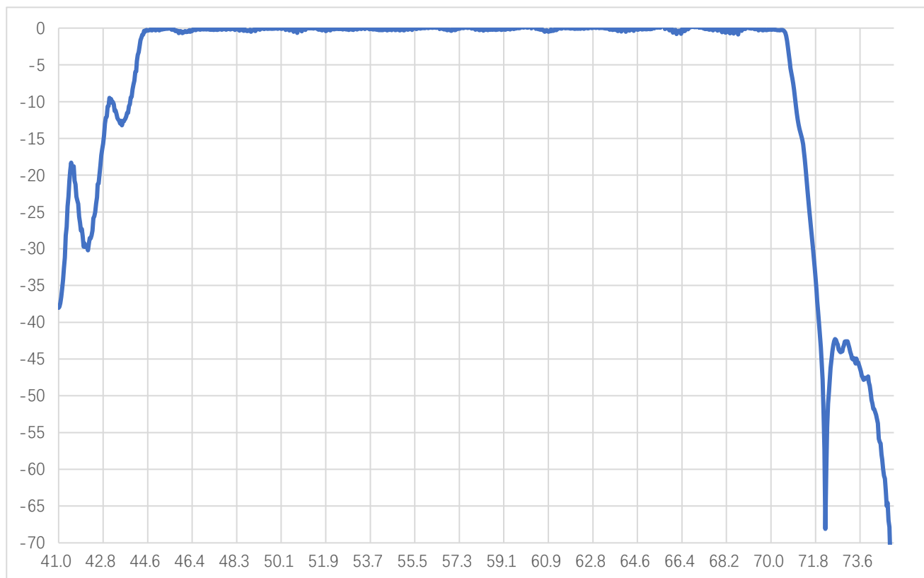
S21 vs Frequency
